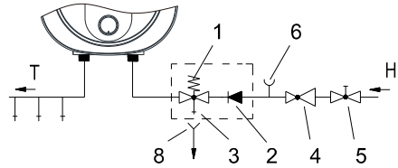
Installation above the basin/sink
