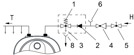
Installation below the basin/sink
