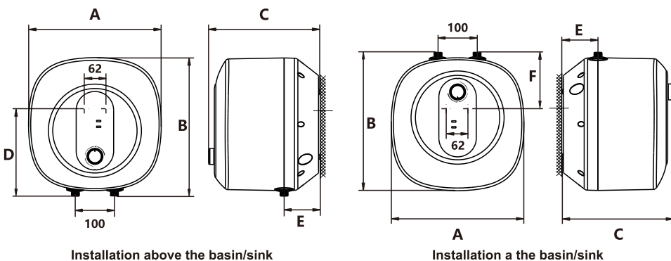
Dimensions of the water heater for installation and connection [mm]
